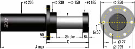
SDP160-F Front Flange
