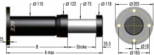
SDP80-R Rear Flange
