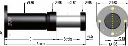
SDP63-R Rear Flange
