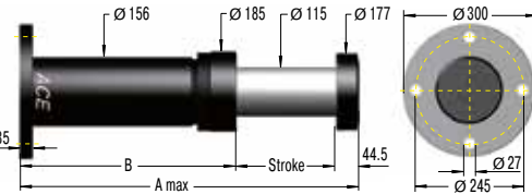
SDP120-R Rear Flange
