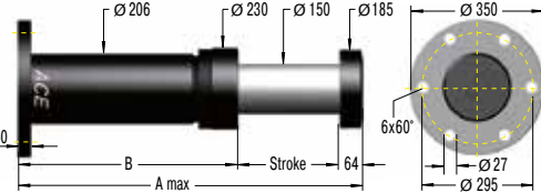
SDP160-R Rear Flange
