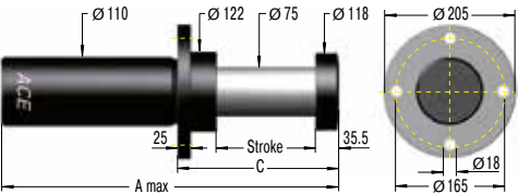
SDP80-F Front Flange
